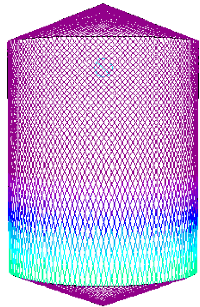
D21.3m (840"), H34m (1,340"), 2xØ11.11mm (2xØ7/16") Time = 24 min.
